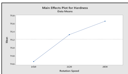
Fig 7: Main Effects Plot for Hardness Vs Rotation Speed
