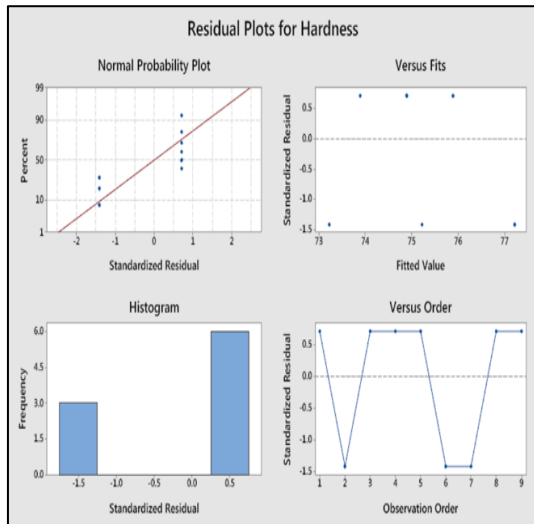
Fig 10: Residual Plot for Hardness
